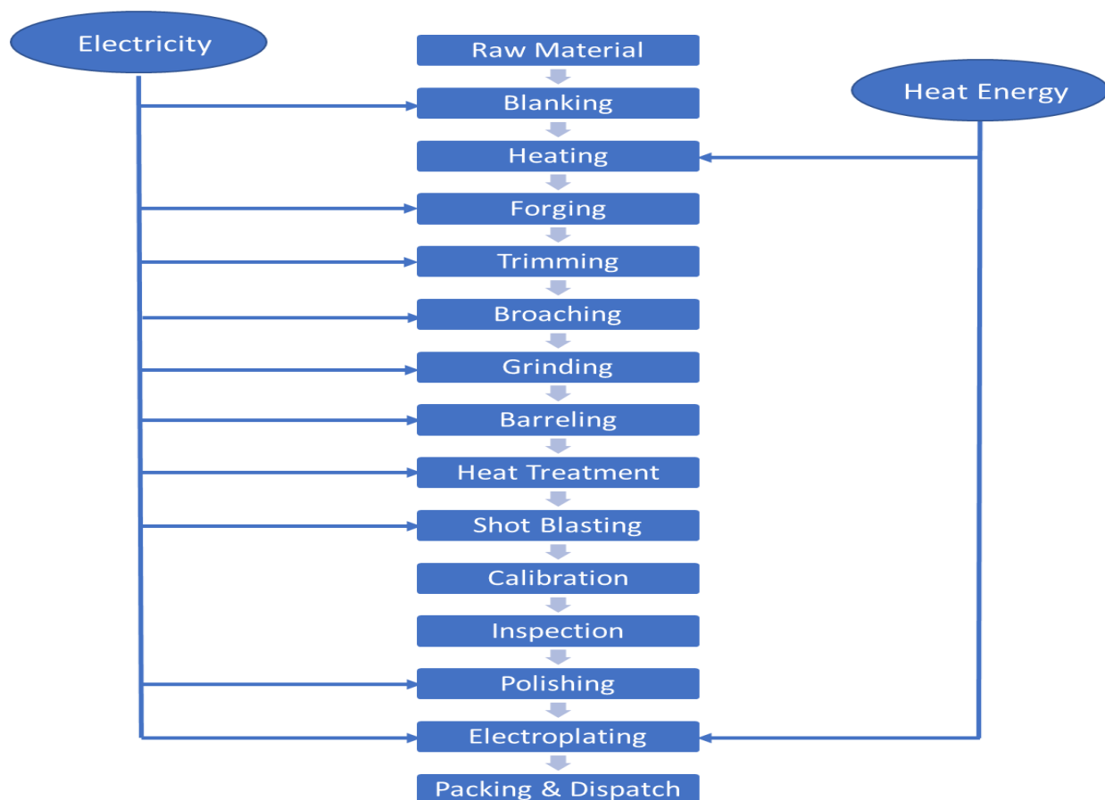
Figure 3: Major Operations in Hand Tool Units
